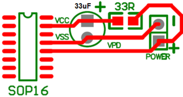
SOP16 PCB layout Diagram:
